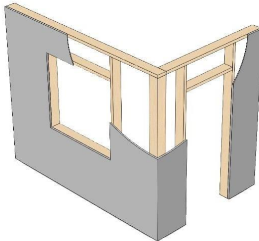
Fig. 1.7. Principle drawing of prefabricated wood elements (InnoBYG, 2017).
