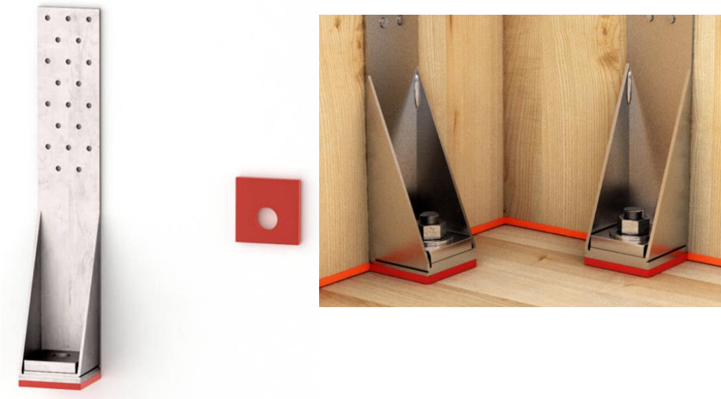
Fig. 3.25. Separating washer for WHT angle bracket (Rothoblaas, 2020)
