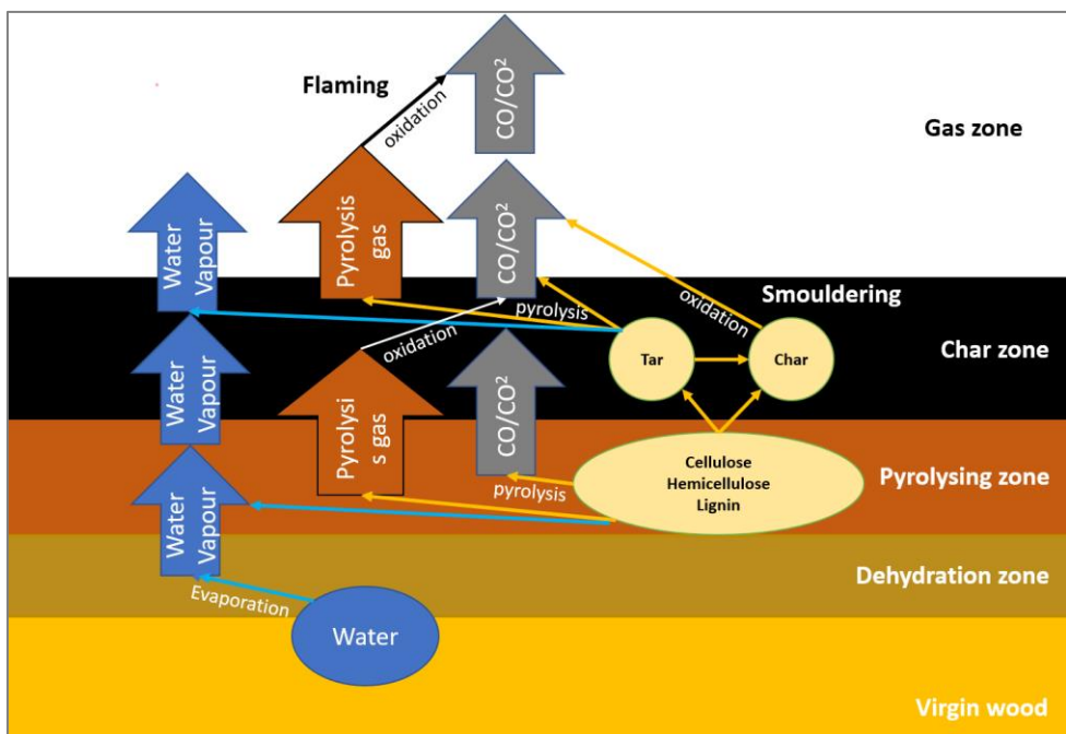
Fig. 3.18. Processes within a burning timber (modified from Bartlett et al., 2019).
