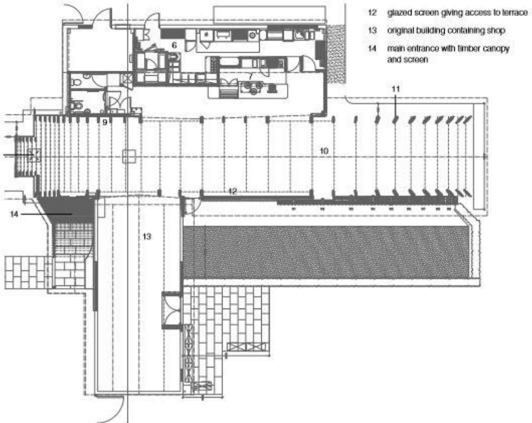
Fig. 7.24. Site and ground floor plan (TRADA, 2019)
