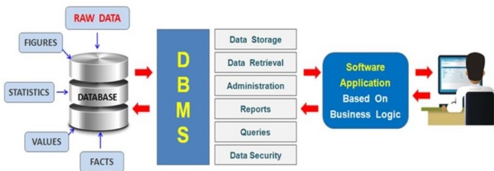
Fig. 6.29. DBMS database management system (Learn Computer Science, 2020).
