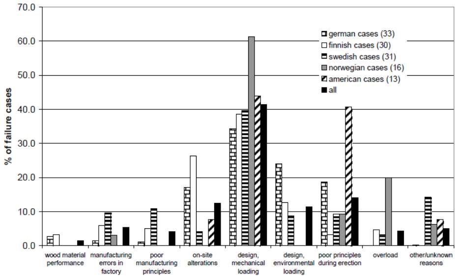
Fig. 6.42. Failure causes depending on country (Frühwald et al., 2007).
