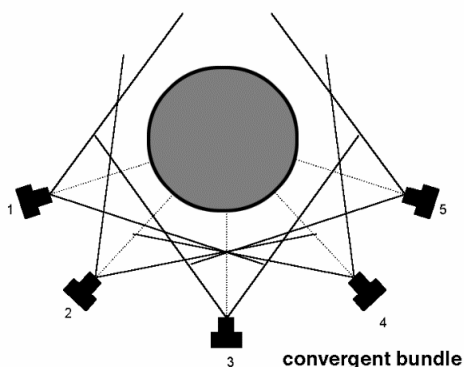
Fig. 6.8. Basic principle for taking the photography (Hanke, 2002).
