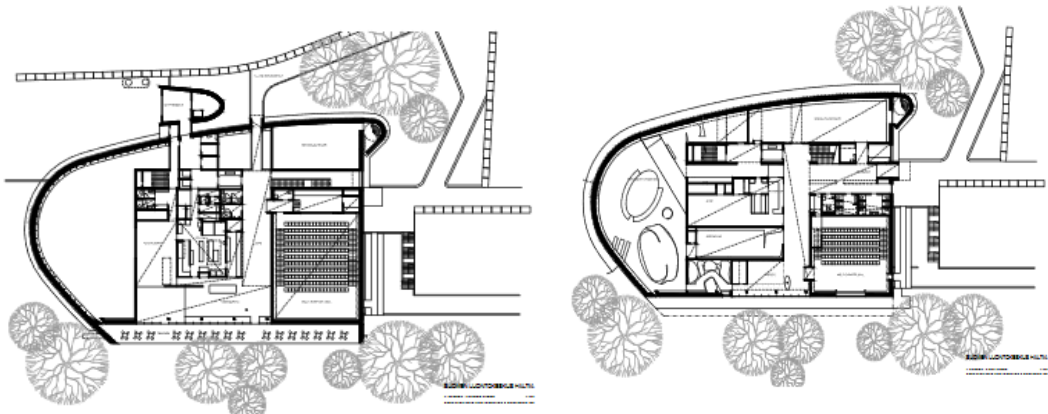
Fig. 7.43. The floor plans. Starting from the top left: second floor, first floor, and ground floor (Mahlamäki, 2013, p. 11)
