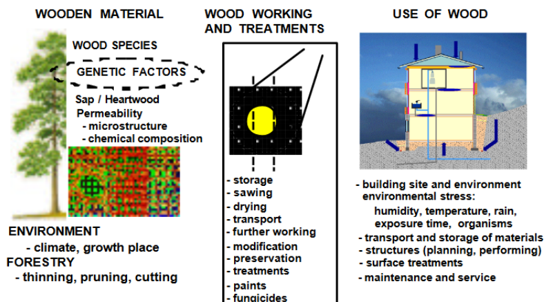
Fig. 3.15. Factors affecting durability of a wooden product (Viitanen et al., 2006).
