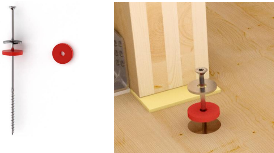
Fig. 3.24. Wood screws separating washer (Rothoblaas, 2020).
