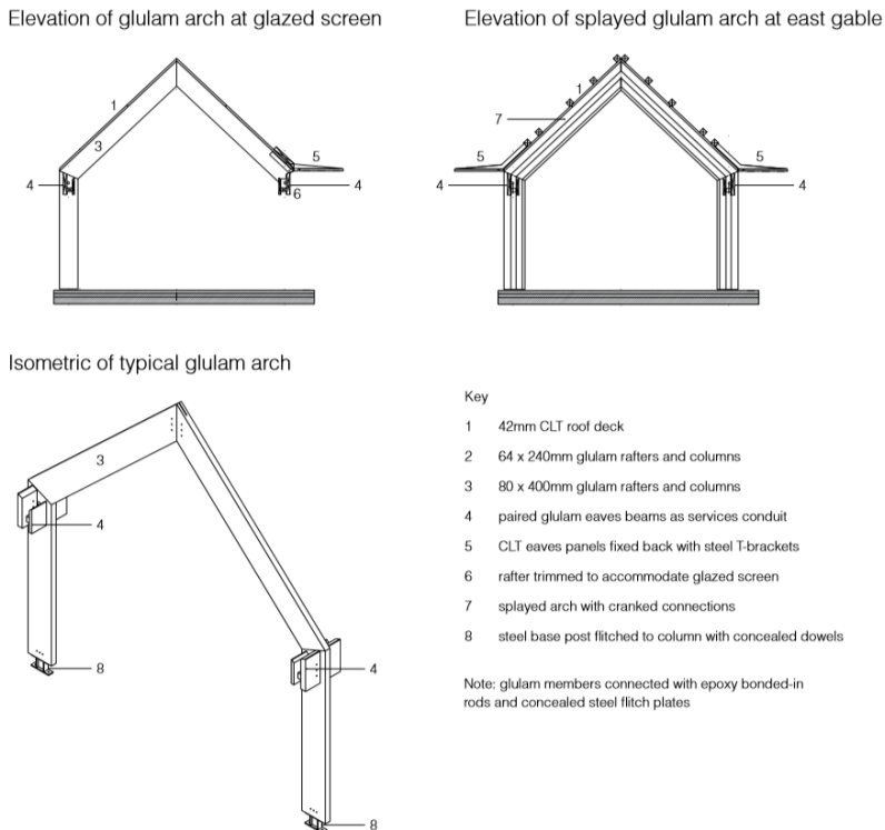
Fig. 7.25. Structural and detail representation (TRADA, 2019)
