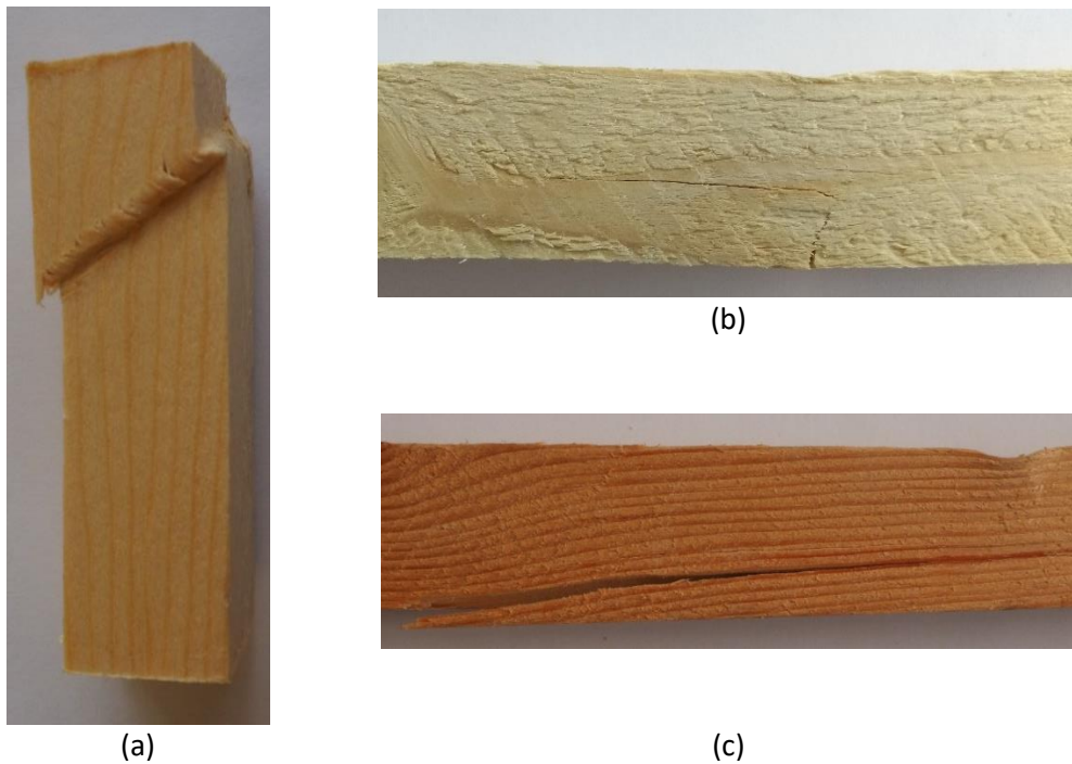
Fig. 2.17. Different failure modes: (a) compression parallel to grain, (b) bending failure, (c) bending failure in the presence of inclined grain.
