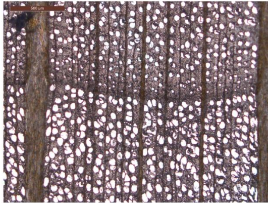
Fig. 2.9. Transverse section through beech. Morwenna Spear© Chris Miles.
