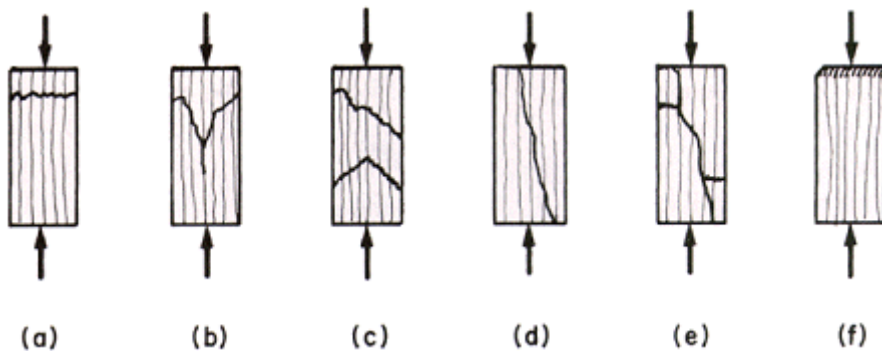
Fig. 6.34. Failure types of nonbuckling clear wood in compression parallel to grain: (a) crushing, (b) wedge splitting, (c) shearing, (d) splitting, (e) crushing and splitting, (f) brooming or end rolling (Bodig & Jayne, 1993).
