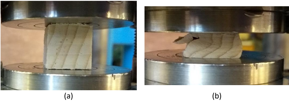
Fig. 2.15. A wood specimen subjected to compression perpendicular to the grain: (a) before testing, and (b) afterwards.
