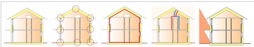
Fig. 1.32. Passive House design principles (Bootland, 2011).
