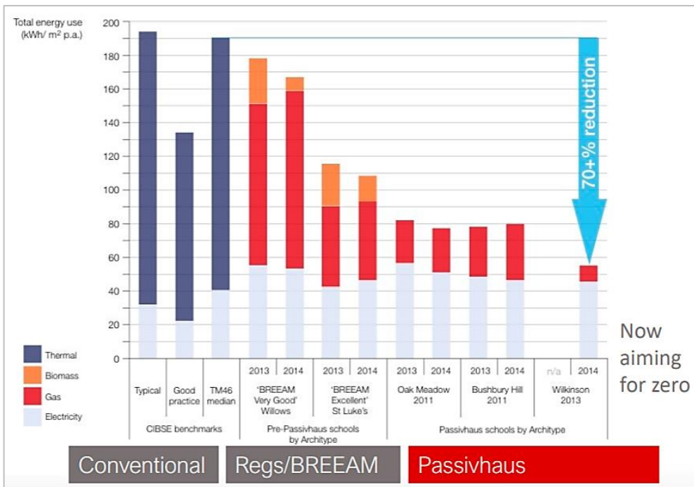
Fig. 1.38. Recorded total energy consumption (Passivhaus Trust, 2020).
