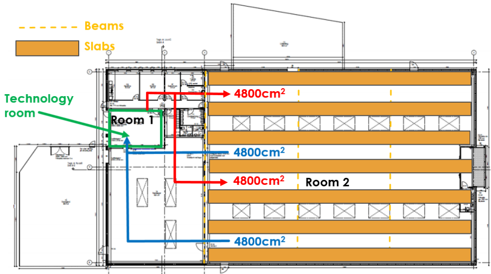
Fig. 3.40. Load-bearing slabs laid at a distance.
