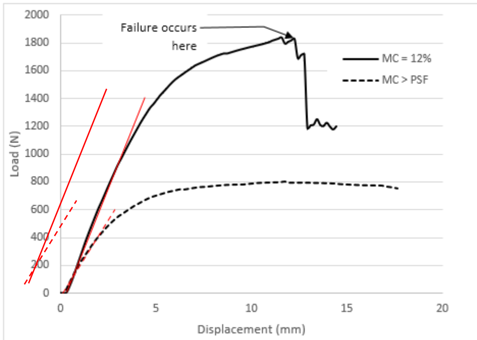
Fig. 2.13. Comparison of bending test results for dry and wet timber.
