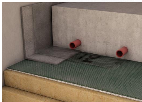
Fig. 3.29. A resilient under screed membrane made of foil and closed cell PE (Rothoblaas, 2020).
