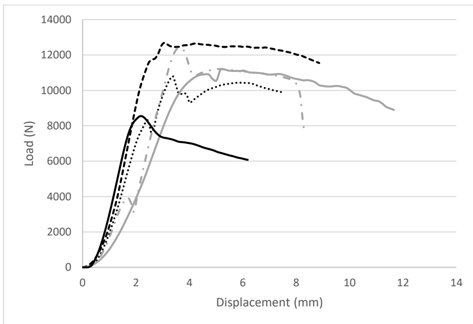
Fig. 2.23. Load-deformation graph for five clear wood specimens subject to compression parallel to grain.
