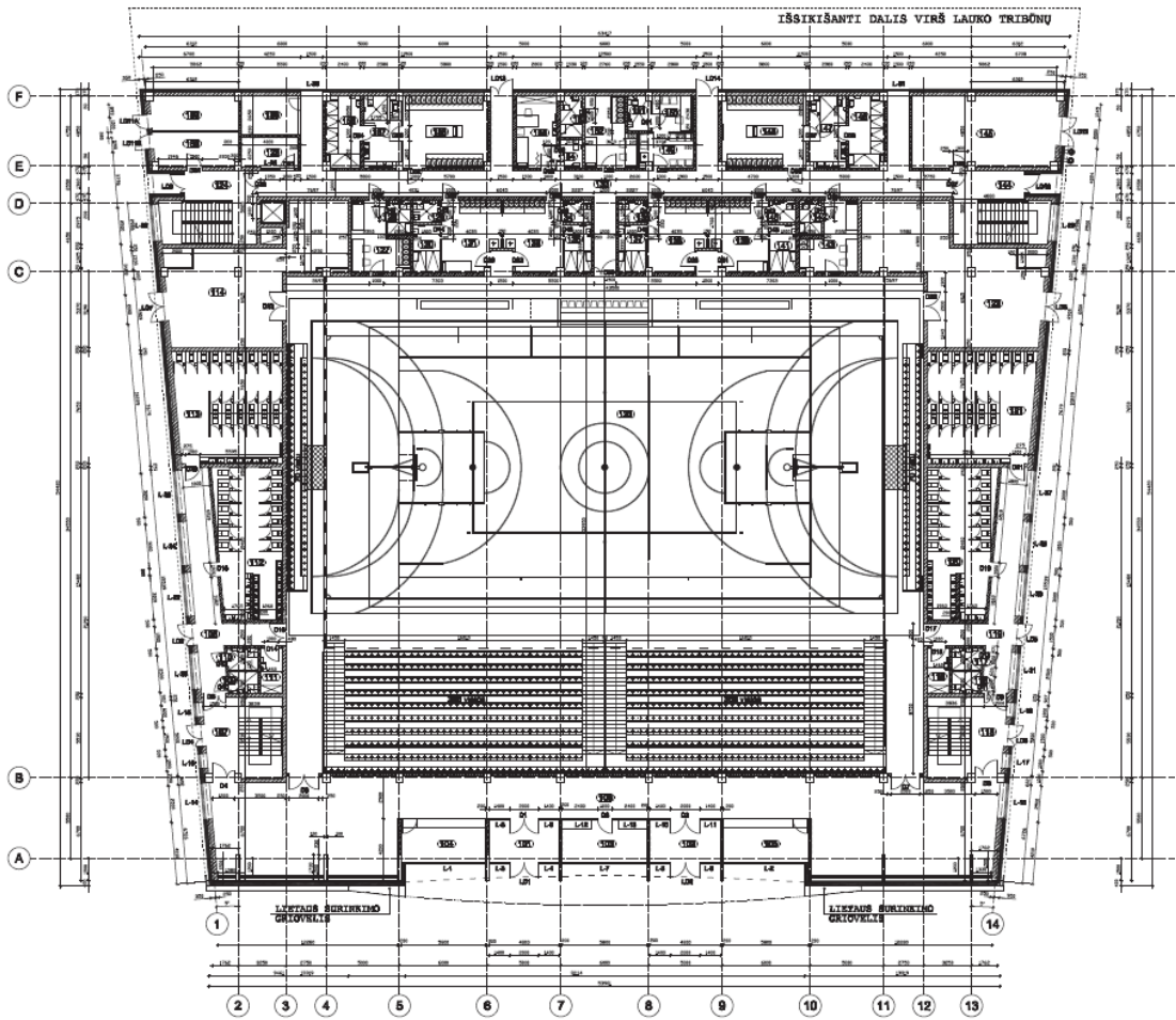
Fig. 7.18. The plan of multifunctional sports hall
