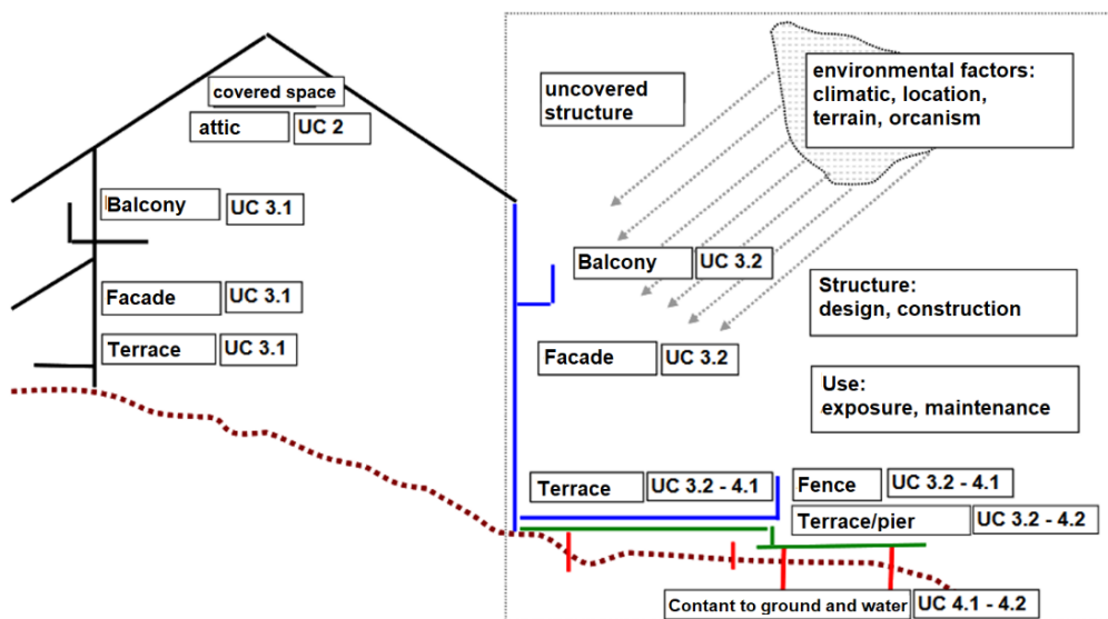
Fig. 3.14. Structures and use class examples (Adapted and translated from (Viitanen, 2004)).
