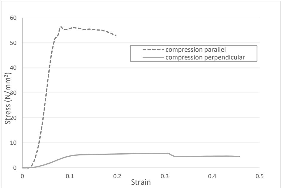
Fig. 2.16. Graph representing stress-strain behaviour for wood in compression parallel and perpendicular to grain.
