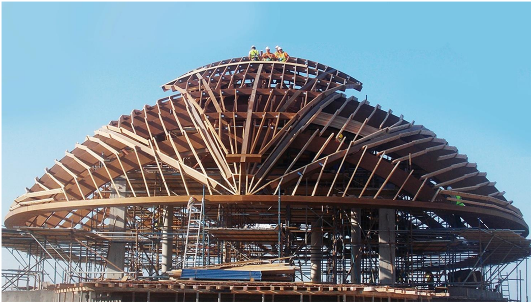
Fig. 7.59. Construction process of the lookout restaurant in Banana Island, Doha, Qatar
