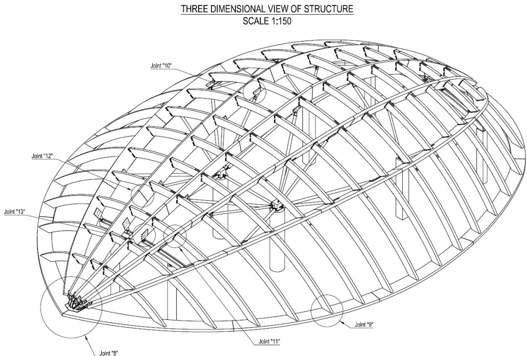
Fig. 7.58. The 3 dimensional view of the lookout restaurant in Banana Island, Doha, Qatar
