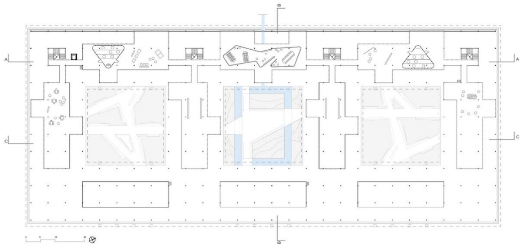
Fig. 7.52. First floor plan (Leonardo Finotti - www.archdaily.com )
