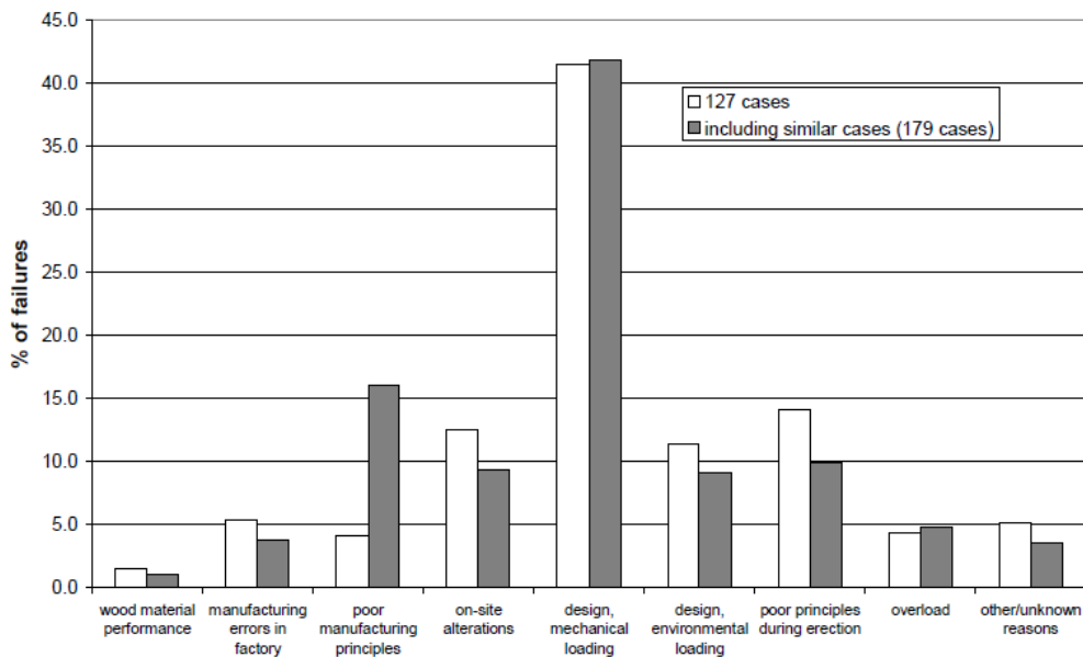
Fig. 6.41. Distribution of error types for the cases in the data base with or without including parallel cases (Frühwald et al., 2007).
