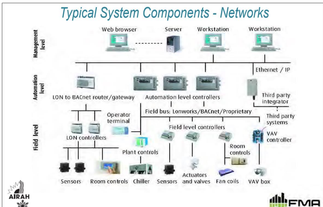
Fig. 6.24. BMS system’s components – network example (City of Melbourne, 2020).
