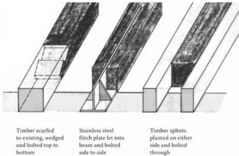
Fig. 6.33. Typical solutions where a beam end has decayed (Russell, 2020).
