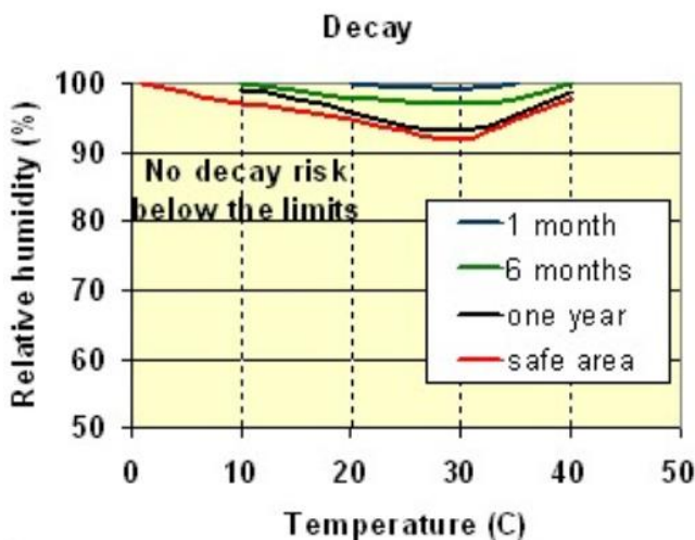
Fig. 3.10. Dependency of decay of wood on temperature and relative humidity.
