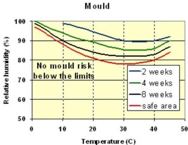
Fig. 3.9. Mould growth dependency on temperature and relative humidity (Viitanen, 2008).
