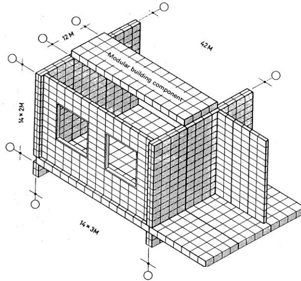
Fig 3.1. All building components in this model are correctly located in their modular zones within the modular space grid. However, technical detailing of the connections usually leads to the grid being broken in several places (Nissen, 1972).
