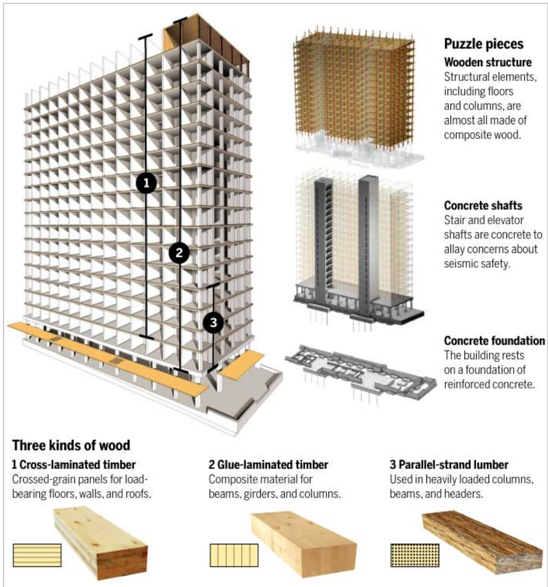
Fig. 1.11. Hybrid construction – Brock Commons (University of British Columbia and Acton Ostry Architects Inc., n.d.).
