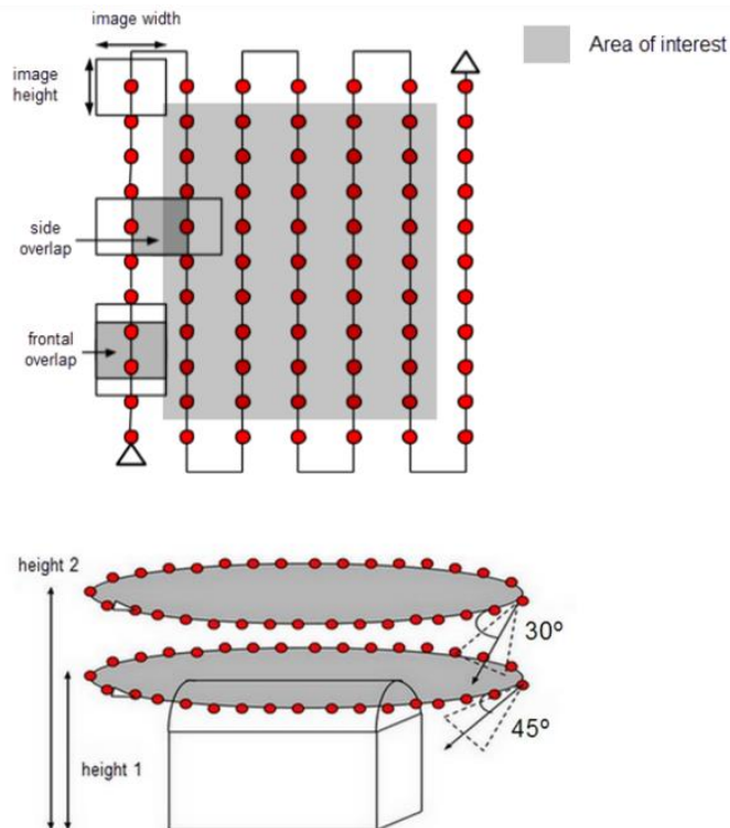
Fig. 6.9. UAV trajectories (Pix4D manuals, 2020).
