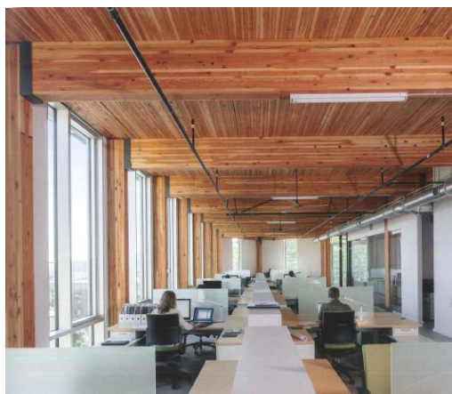
Fig. 3.39. Ventilation ducts under the load-bearing beams.
